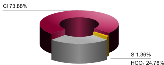
Anion Balance (%)
