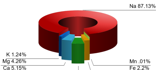
Cation Balance (%)
